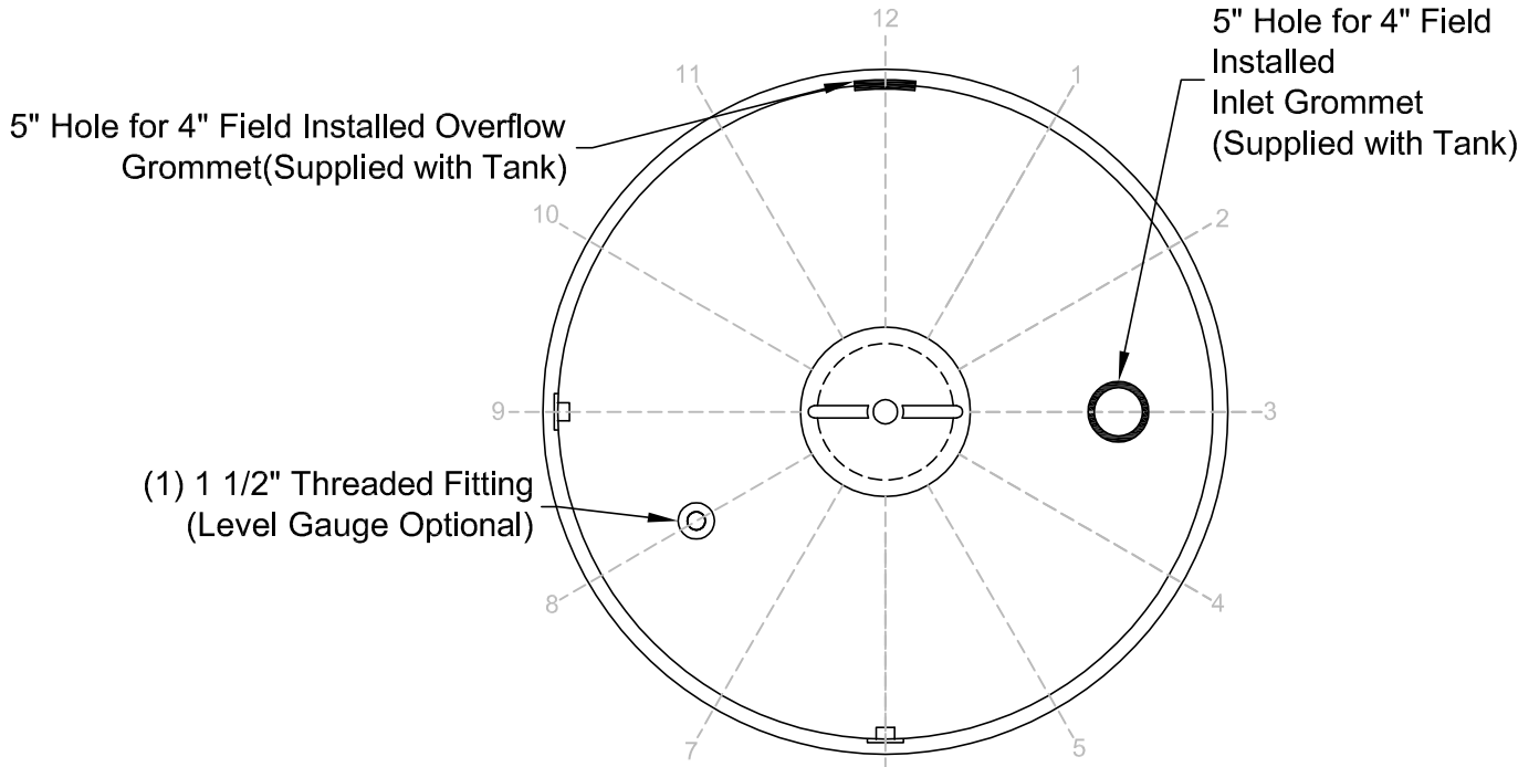
TOP VIEW 14" O.D. Access Lid (11 1/4" I.D. Opening)
