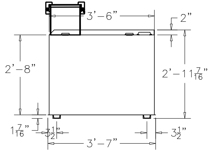
END VIEW
