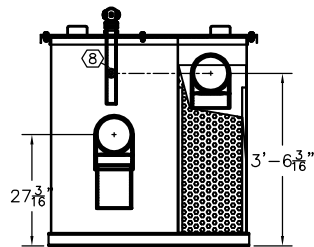
LEFT END VIEW
