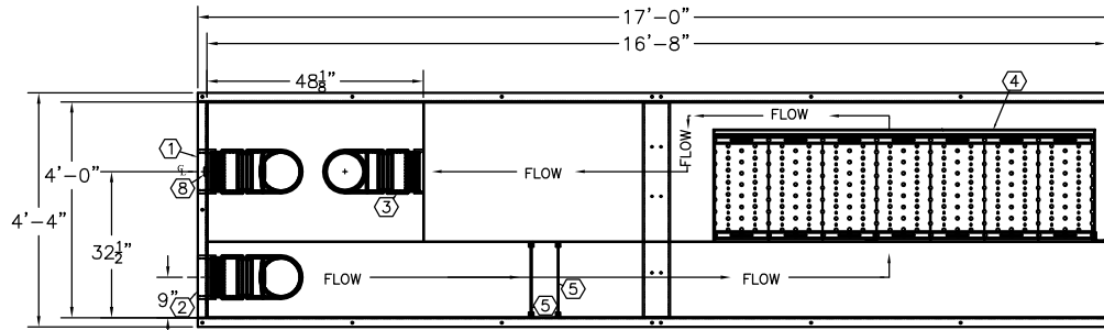
TOP VIEW TOP COVER REMOVED FOR CLARITY REFER TO DWG. "CVB006" FOR COVER DETAIL
