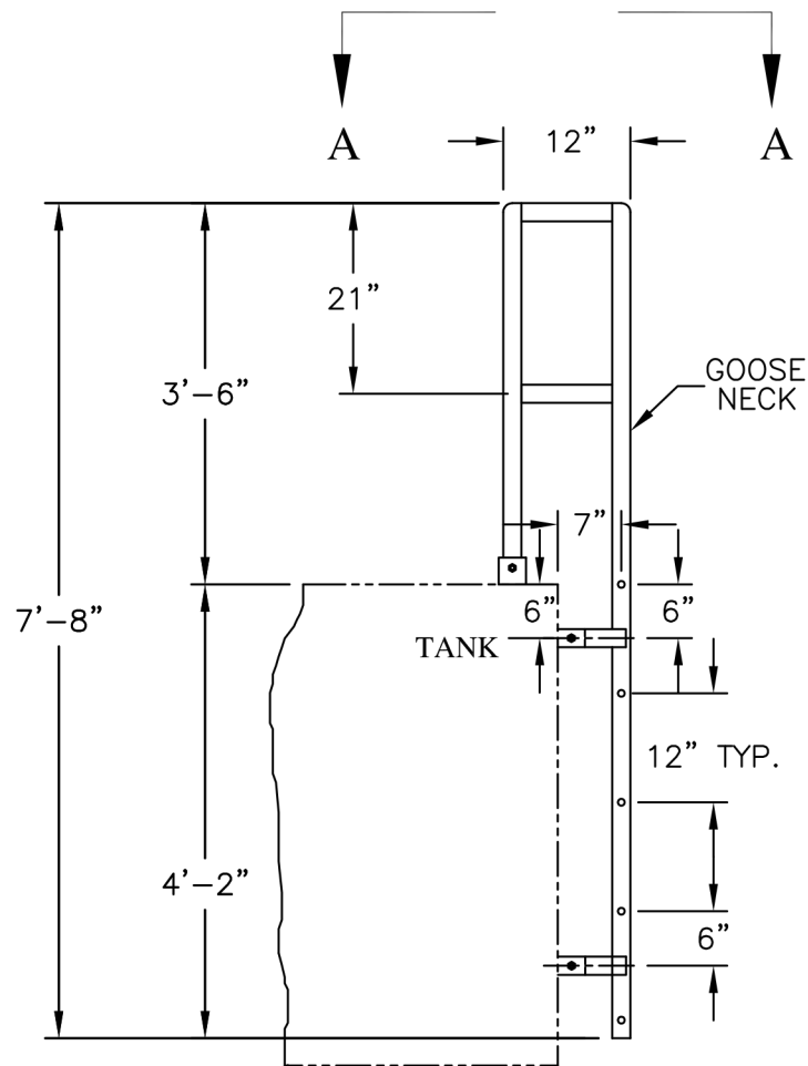
5-RUNG LADDER
