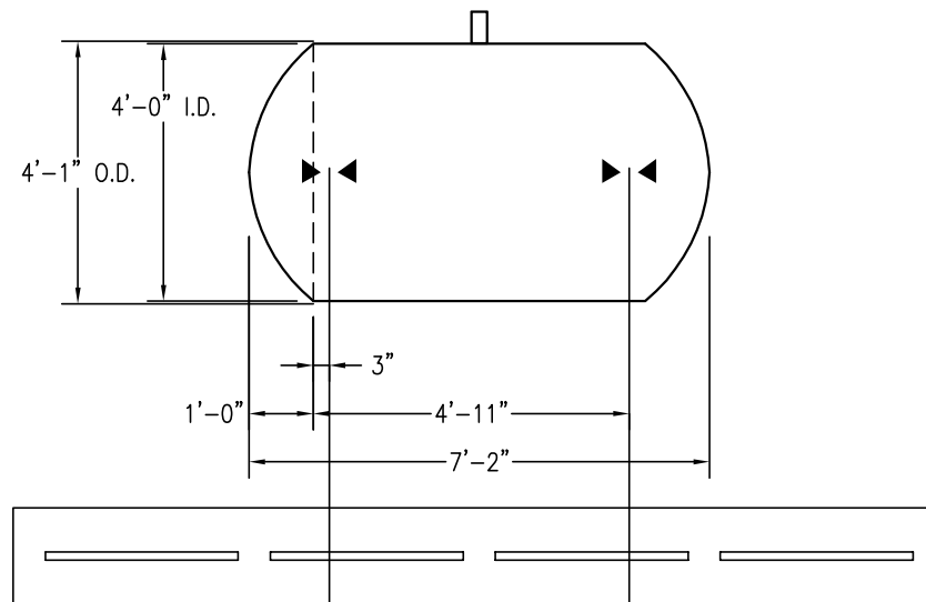
OPTIONAL 18"x 8"x 14' DEADMAN
