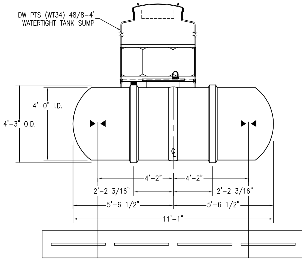
OPTIONAL 18"x 8"x 14' DEADMAN
